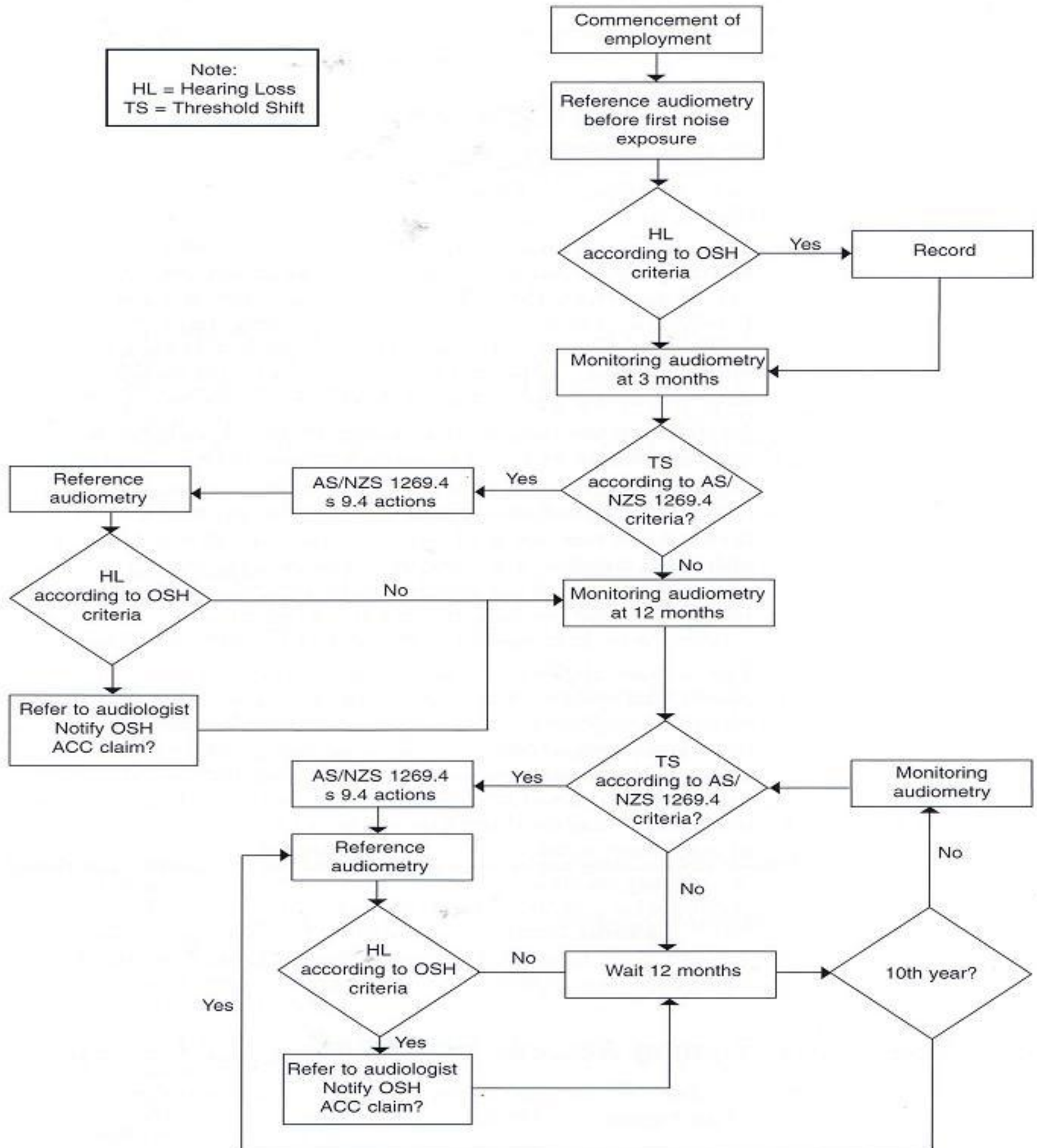
Figure E.2: Flow chart of audiometry testing procedure given in AS/NZS 1269.4
